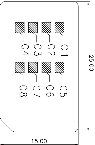
REFERENCE SIM CARD PLUG
