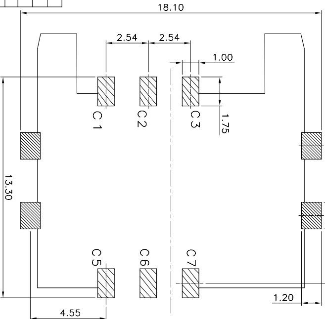
RECOMMENDED PCB LAYOUT GENERAL TOLERANCE ±0.05
